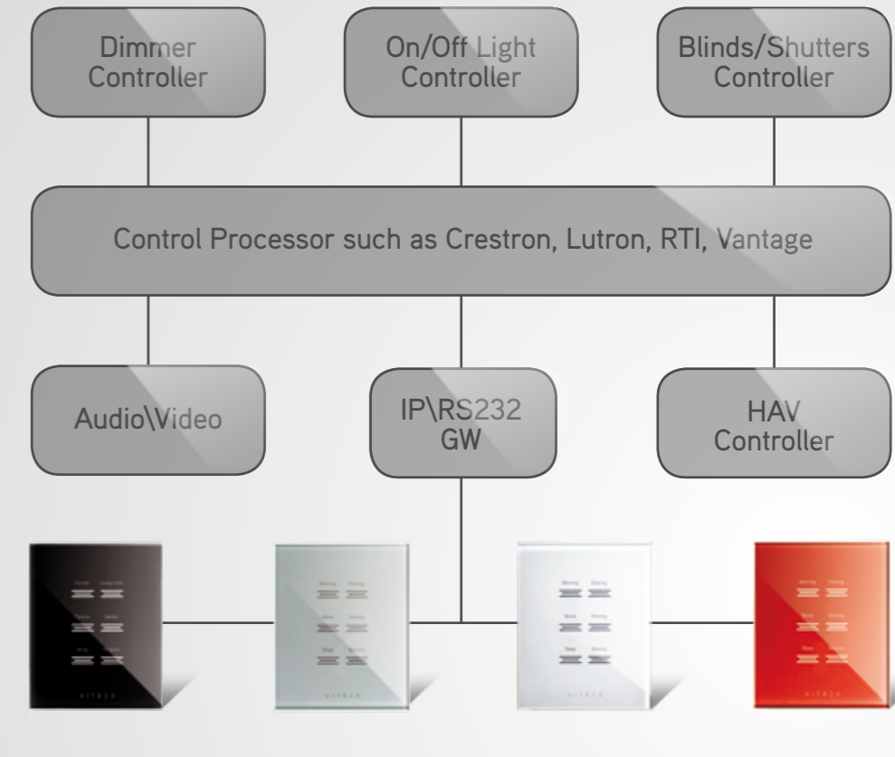
Integration of VTouch Plus Switches with Smart Home Systems
